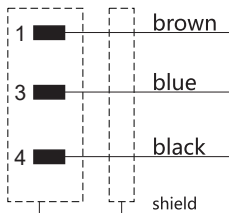
Circuit diagram
